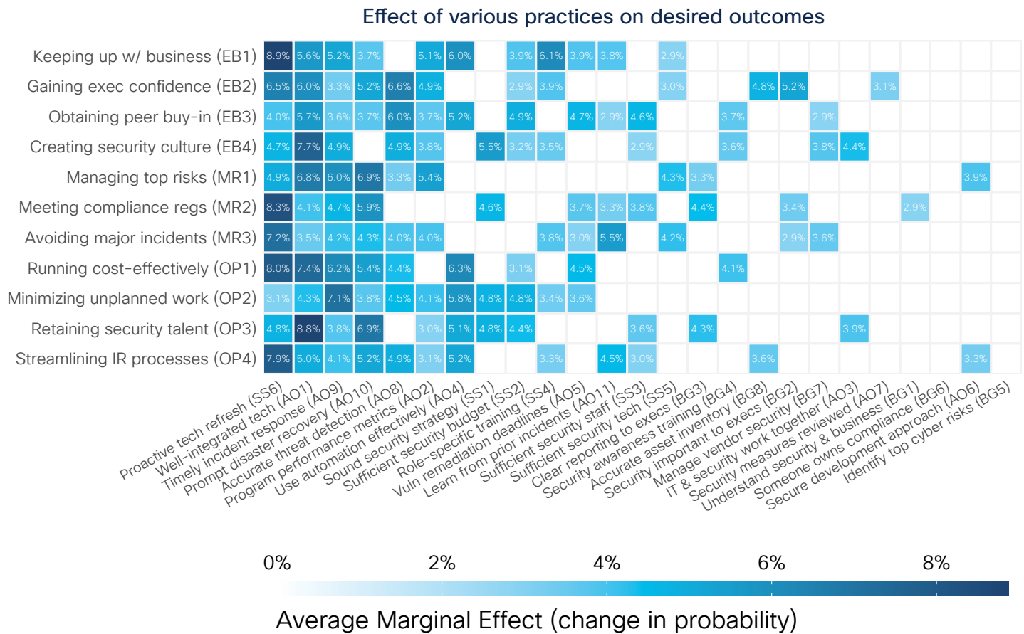
Figure 15: All security practices correlated with each security program outcome
